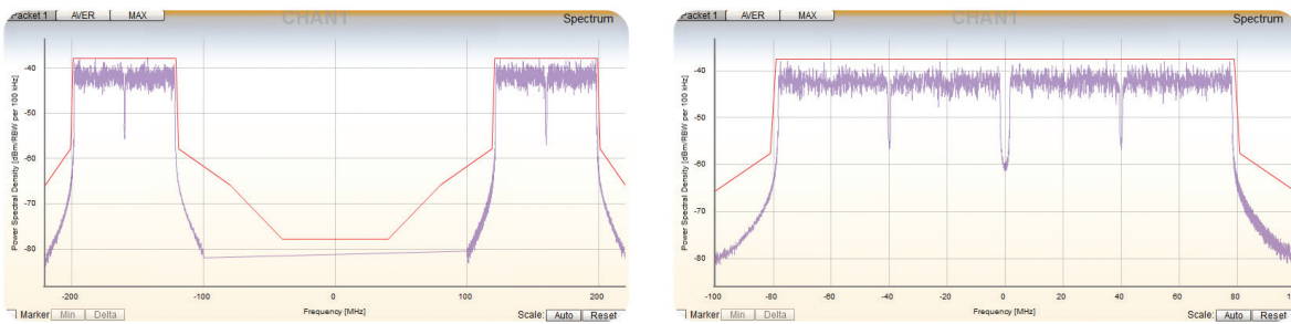
Figure 1: IQxel Test System Mask Testing of 802.11ac 80+80 non-contiguous and 802.11ac contiguous standards
